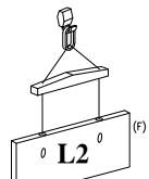
L2 2 WAY EDGE WITH SPREADER OR 2 WAY FACE WITH SPREADER (L2-F)
